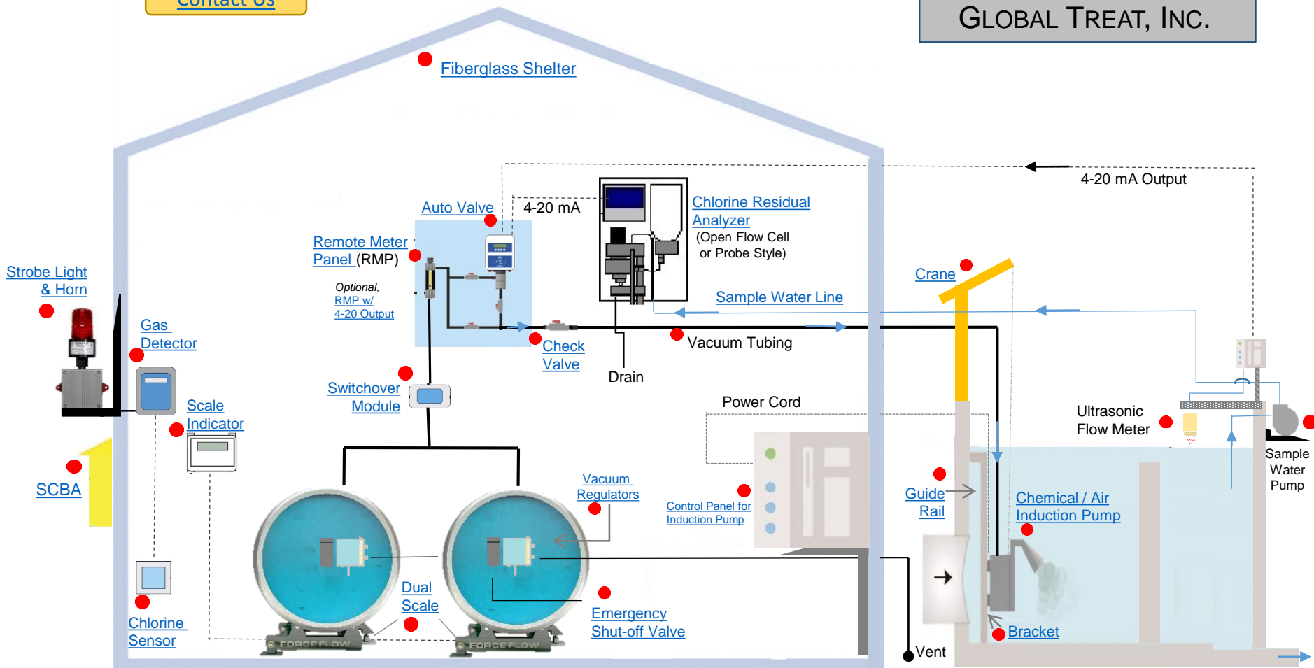
Water Chlorination and De-Chlorination Systems
