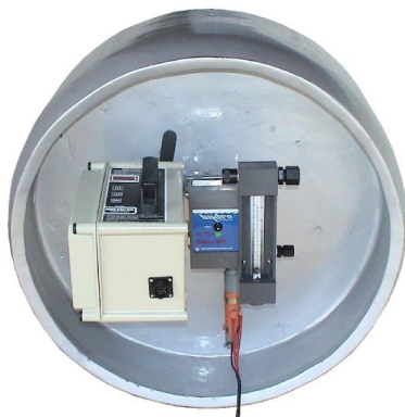
Shut off valve with Vacuum Regulator
